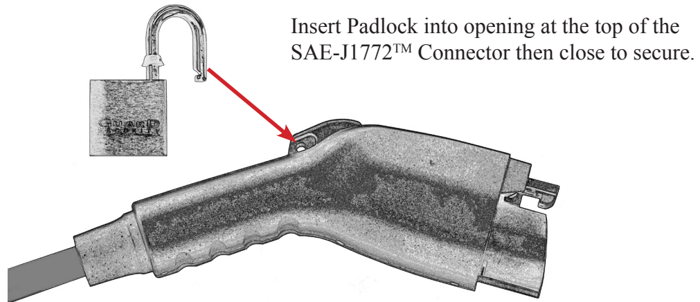
Figure 2. Charge Connector is now secured with Padlock and cannot be removed from vehicle without key.
