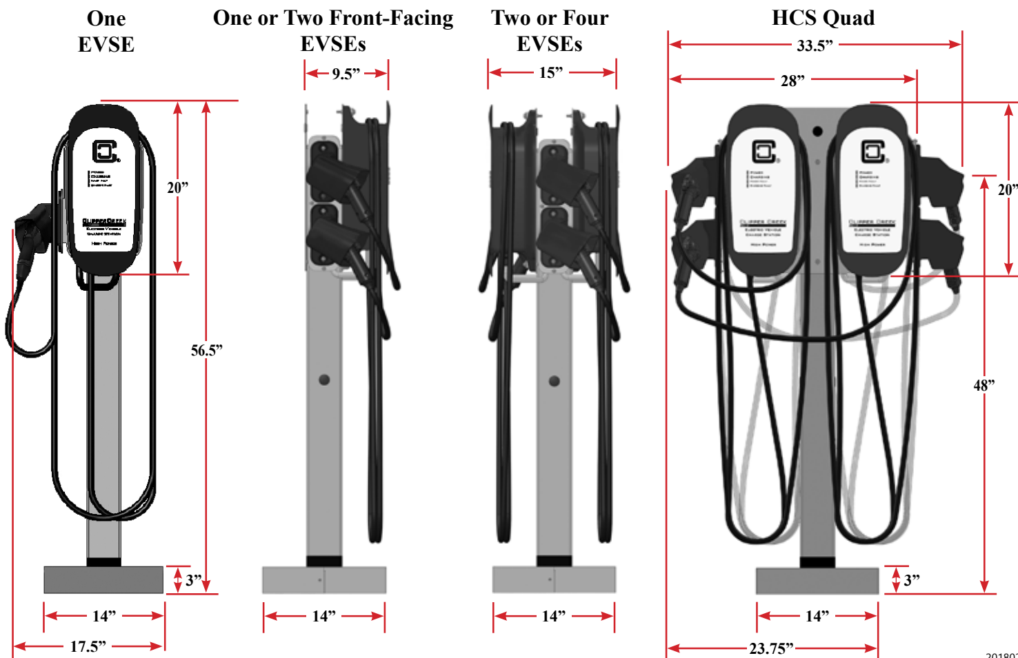
Industry standard bolt pattern and pedestal base dimensions
