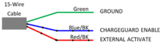
Figure 14: COSMOS ChargeGuard EX Controls: 15 Wire
